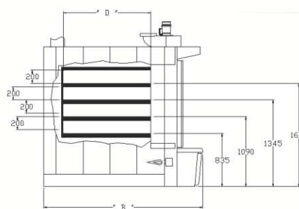
4 camere / 4 chambers
