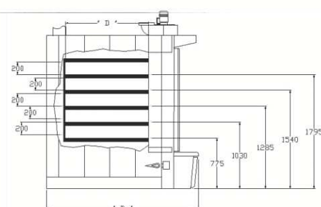
5 camere / 5 chambers
